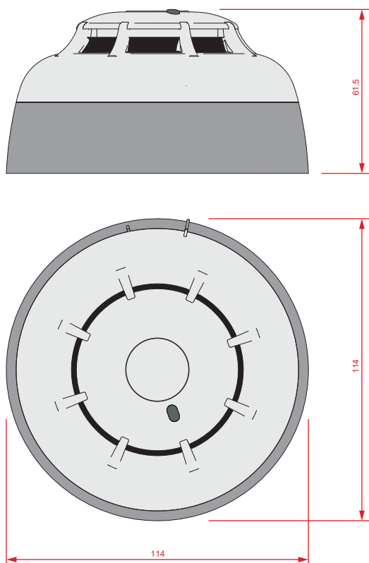
Air2-FD100 - dimensions
