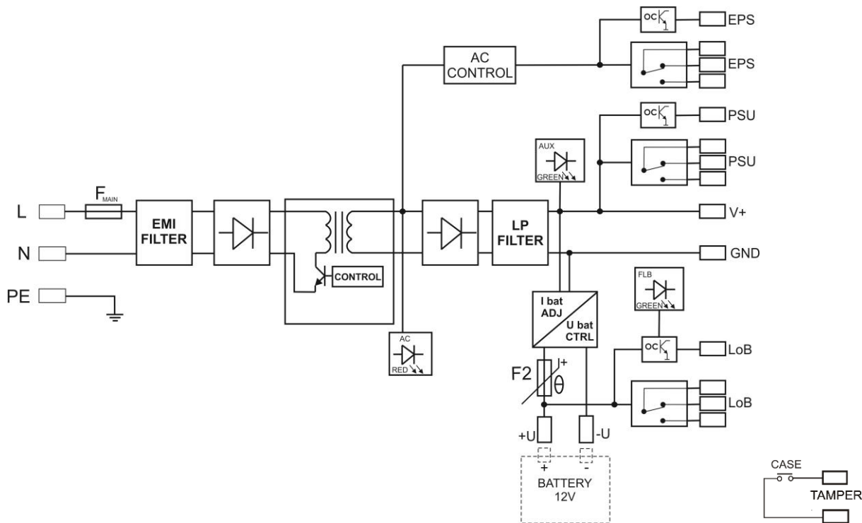
Fig.1. The block diagram of the PSU.
