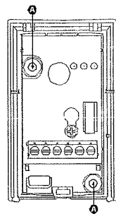
Fig. 2 - Detector installation
