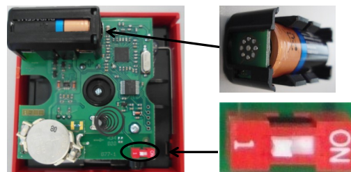
Picture 6 - primary battery, secondary battery, primary battery housing and link-program switch
