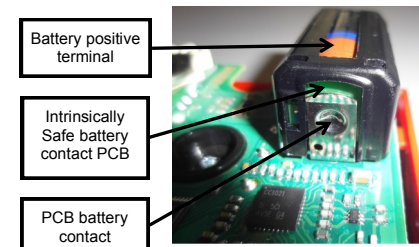
Picture 7 - correct battery insertion
