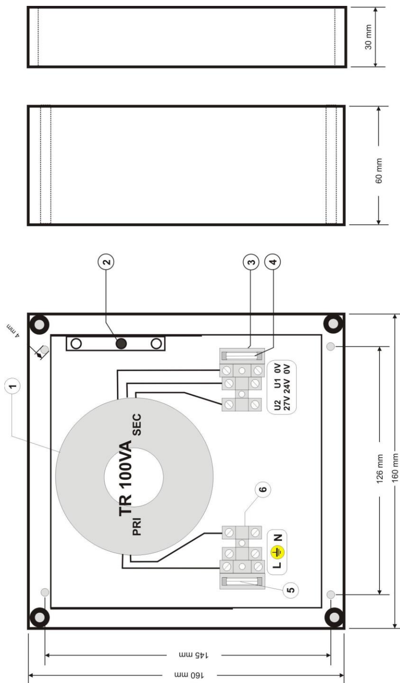
Fig.2. The view of the PSU.
