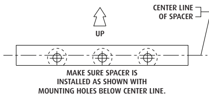
SPACER ORIENTATION
